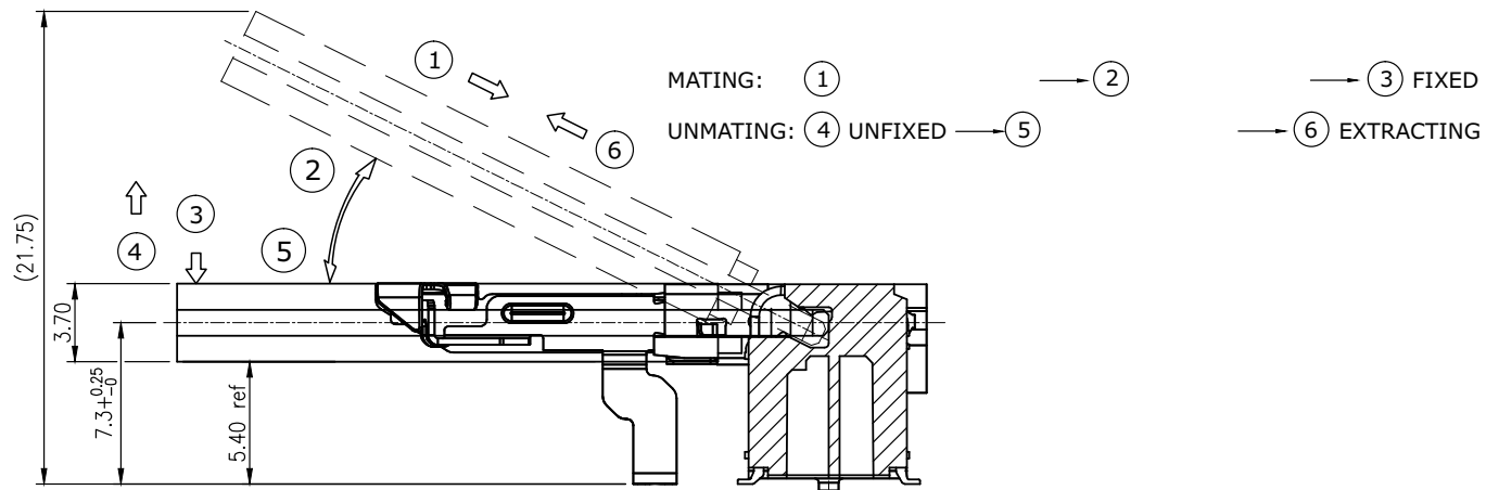
MATING/UNMATING VIEW
