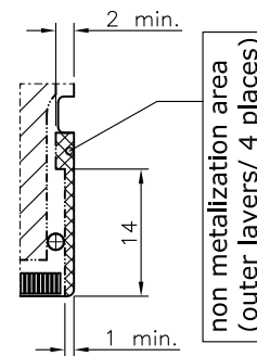
Detail F
