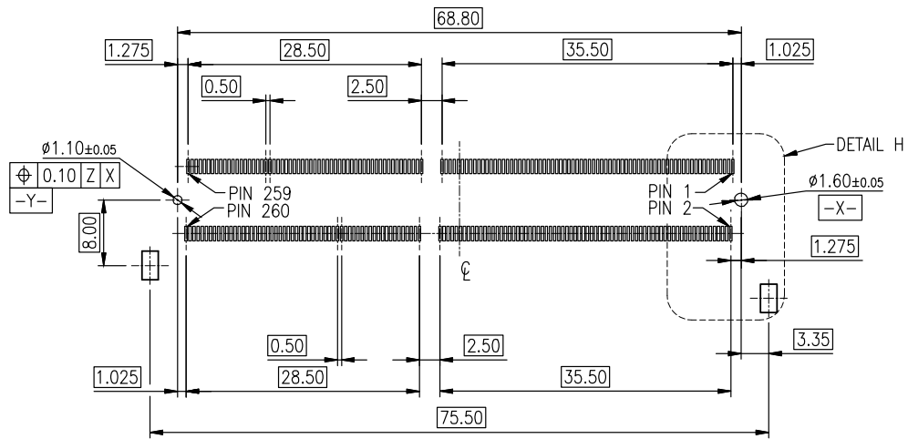
RECOMMENDED LAYOUT (TOP VIEW)
