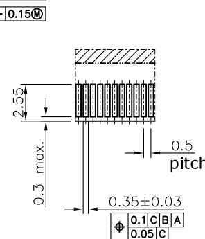
Detail D SCALE 3.125
