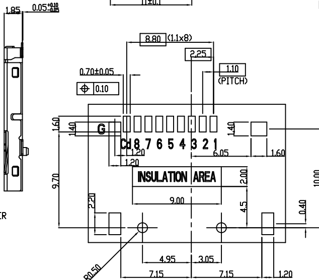
RECOMMEND PC BOARD LAYOUT
