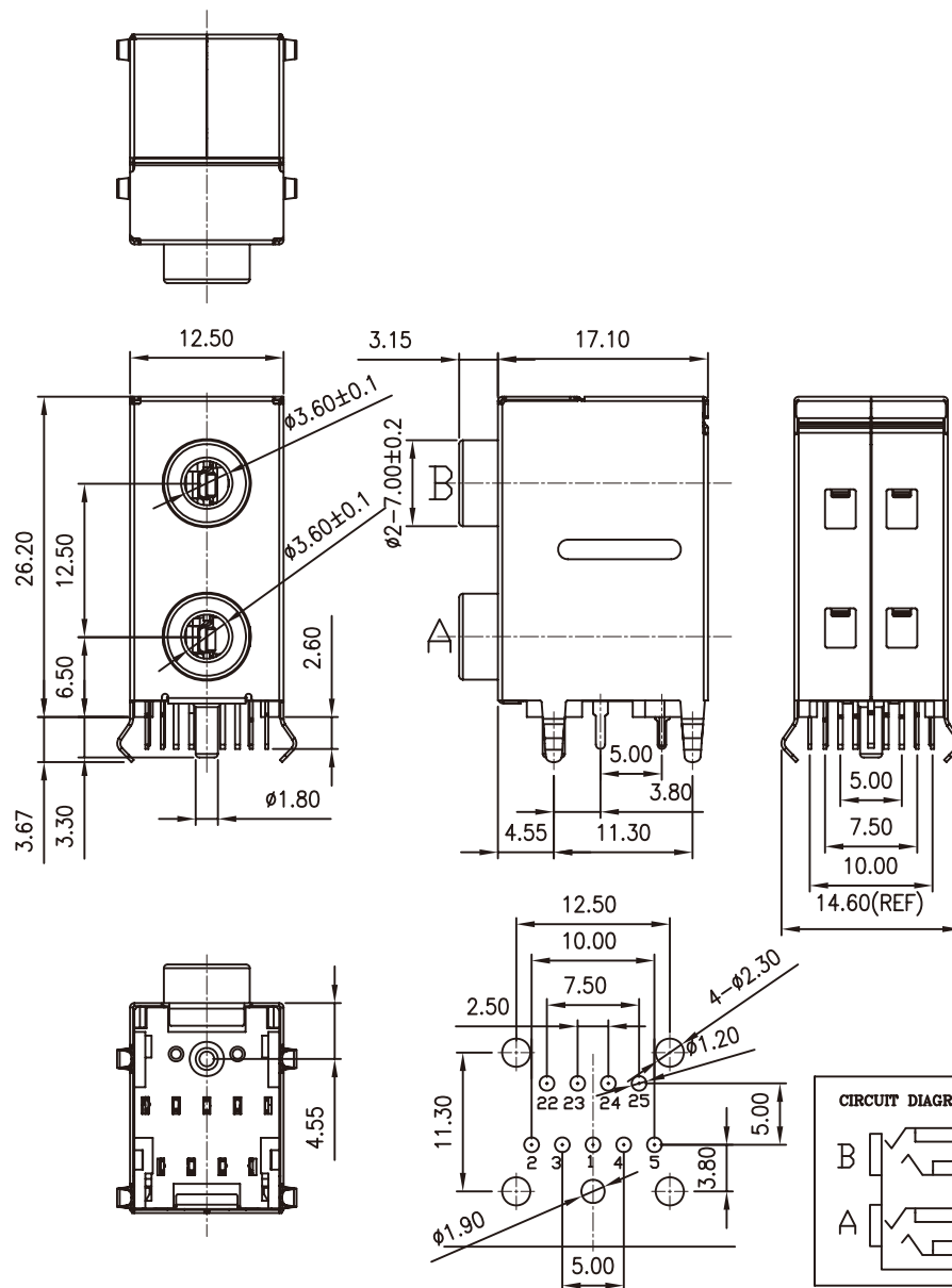
RECOMMENDED PCB LAYOUT
