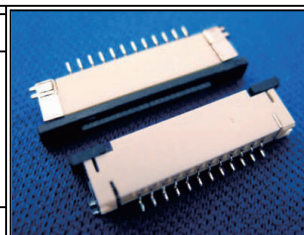
FFC/FPC DIMENSION THICKNESS 0.30±0.03 mm
