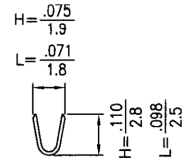
B-B SECTION
