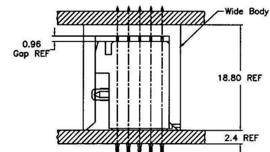
Board-to-Board Offset Application Example
