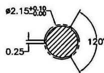
DETAIL J
