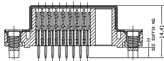
B-B SECTION
