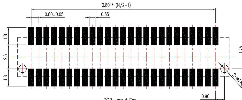
PCB Layout For Surface Mounting
