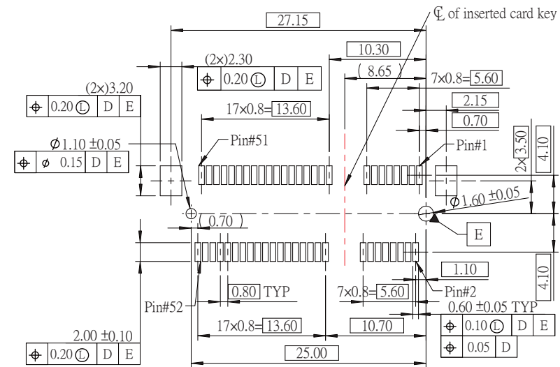
Datum D is the top surface of PCB. RECOMMENDED P.C.B. LAYOUT TOP VIEW(2:1)
