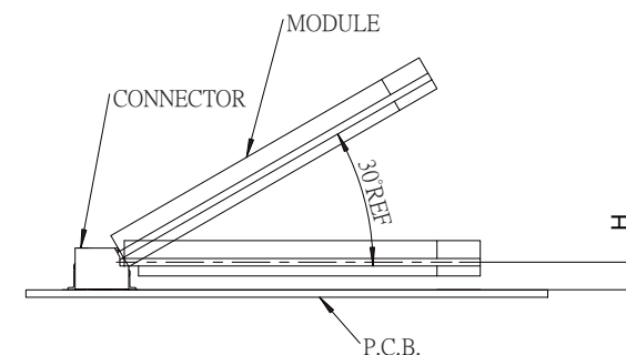
MATING CONDITION
