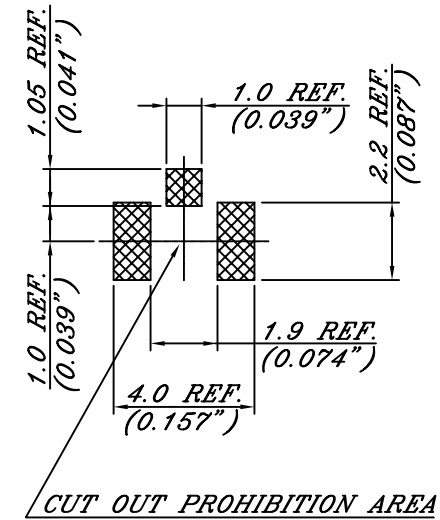
RECOMMENDED P.C.B. PATTERN
