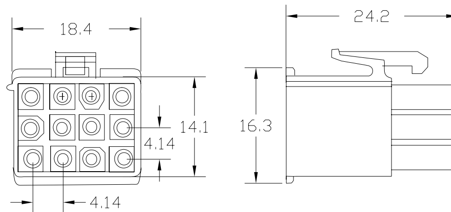
Pcs/1bag ML-S-3X04 500
