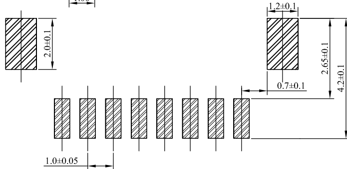
RECOMMENDED P.C. BOARD PATTERN DIM.
