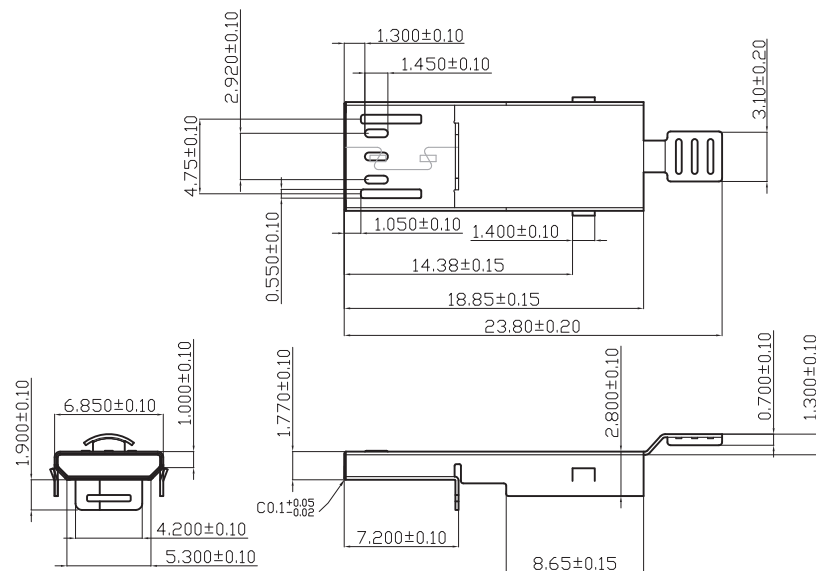
FRONT SHELL
