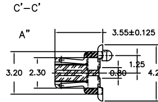
0.80mm(.031")Pitch Board-to-Board Plug
