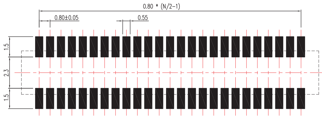
PCB Layout For Surface Mounting
