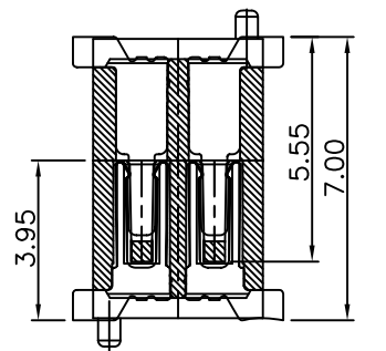
Mating Height Draw
