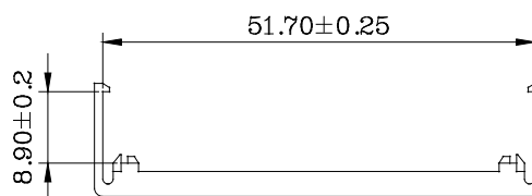
Strain Relief
