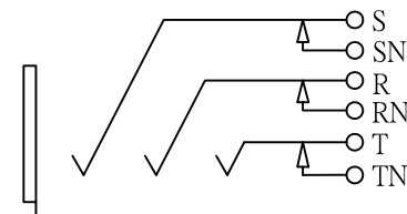
JACK- NORMALLING
