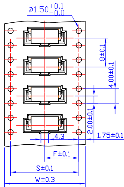
14~16P&20P Contacts
