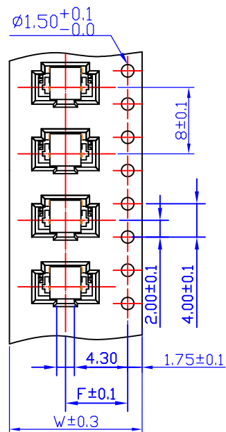
2~13P Contacts
