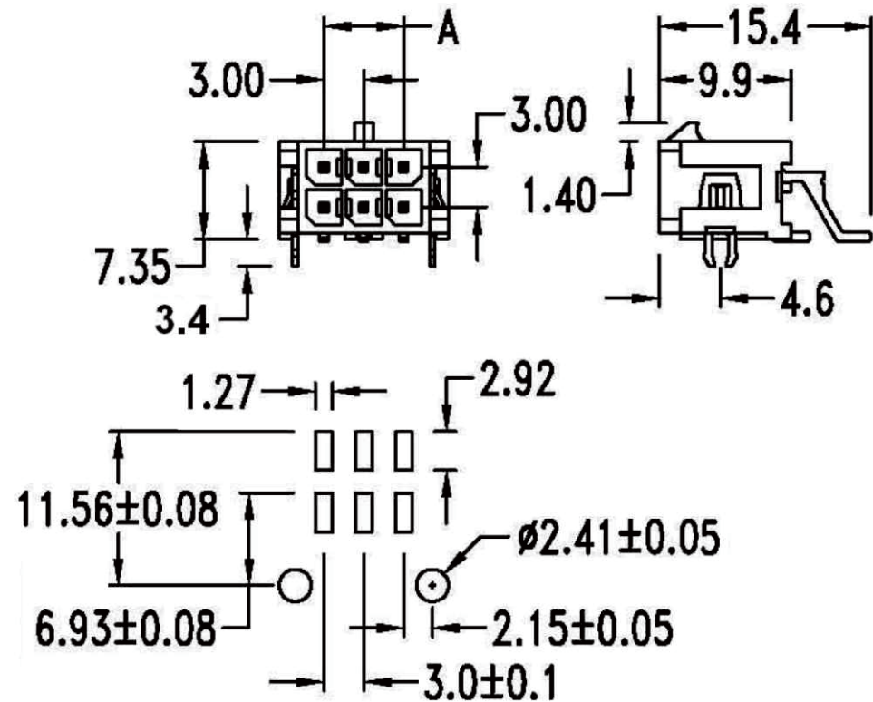
PCB Layout: Component side
