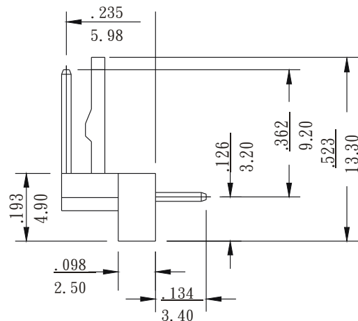
Dimensional information -inch/mm (8812/8813)
