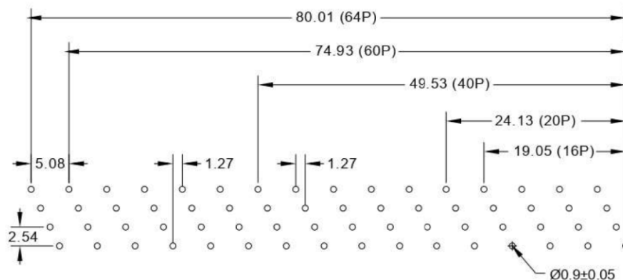
RECOMMENDED P.C.B LAYOUT FOR 16,20,40,60,64
