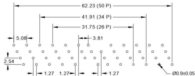
RECOMMENDED P.C.B LAYOUT FOR 26,34,50
