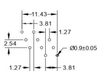
RECOMMENDED P.C.B LAYOUT FOR 10
