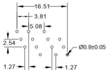
RECOMMENDED P.C.B LAYOUT FOR 14
