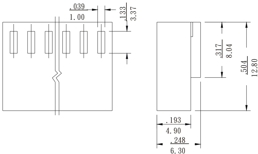
Dimensional information-inch/mm
