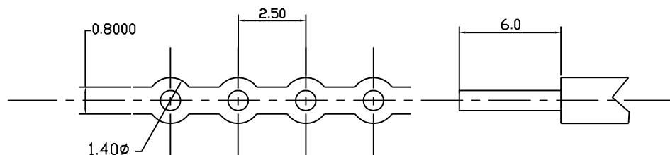
CABLE DIMENSION
