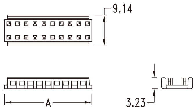
Dimensional Information – in ( mm )
