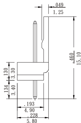
Dimensional information -inch/mm
