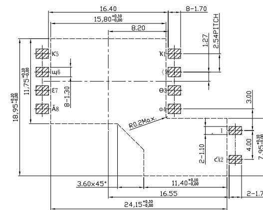
PCB Layout Reference PCB Board B (Inverse)
