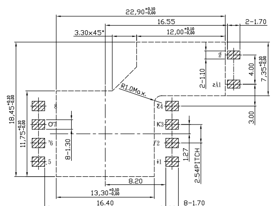
PCB Layout Reference PCB Board A (Frontispiece)
