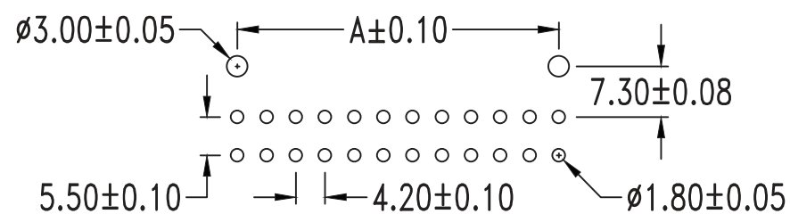
PCB LAYOUT: COMPONENT SIDE
