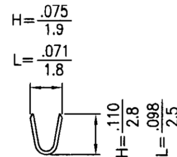
B-B SECTION
