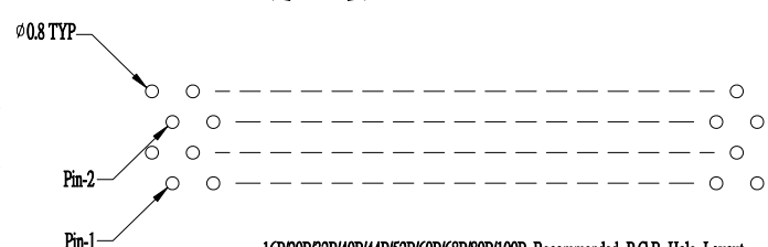
16P/20P/32P/40P/44P/52P/60P/68P/80P/100P Recommended P.C.B Hole Layout
