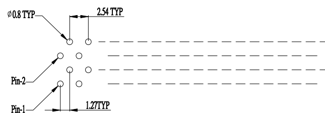
10P/26P/30P/34P/50P/70P Recommended P.C.B Hole Layout
