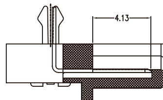
SECT:B-B
