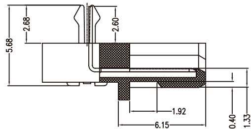
SECT:A-A
