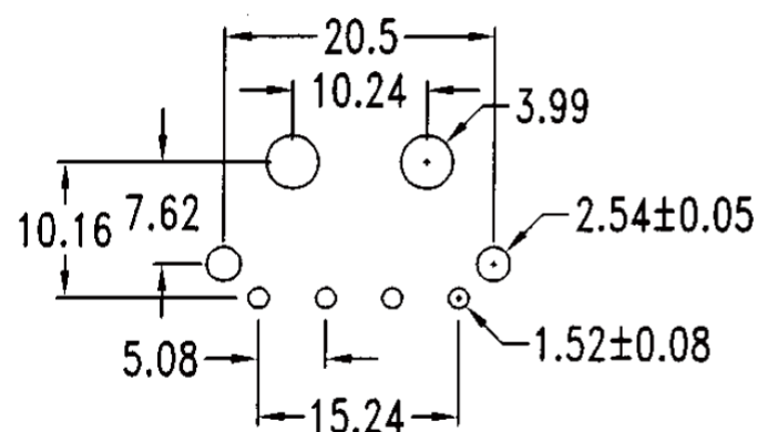
P. C. board hole dimensions
