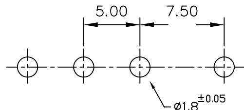
PCB LAYOUT COMPONENT SIDE
