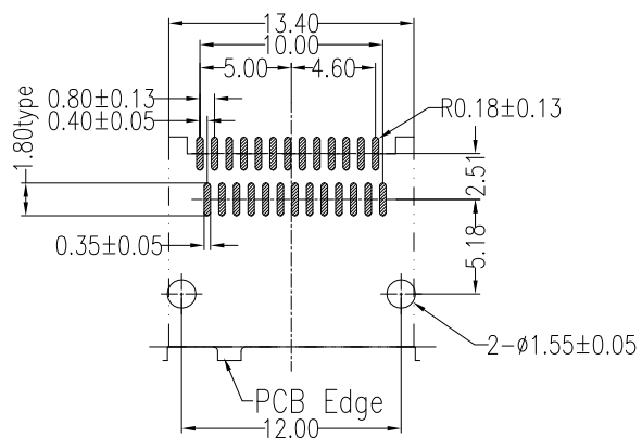
PCB LAYOUT(T=1.60mm) COMPONENT SIDE
