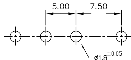
PCB LAYOUT COMPONENT SIDE
