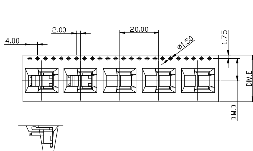
02~03 CONTACTS
