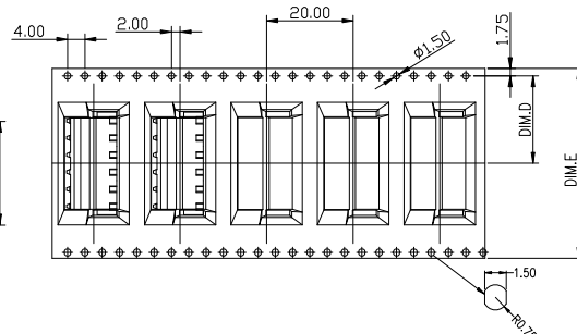
04~06 CONTACTS
