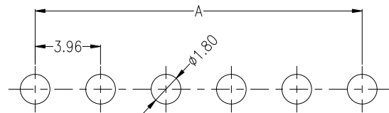
RECOMMENDED PCB LAYOUT(TOP VIEW) TOLERANCE: \pm 0.05\text{mm}
