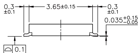
MATED DRAWING(REF.)
