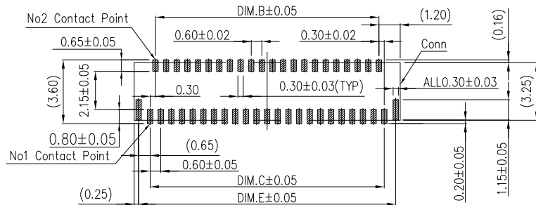
FPC/FFC Insert Direction Recommended P.C.B Layout
