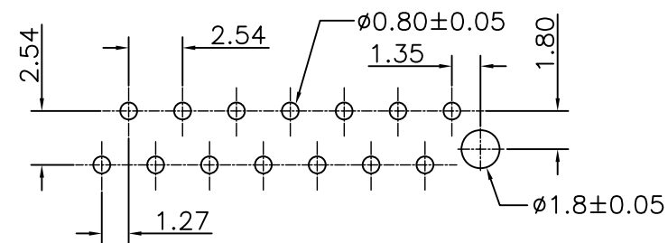
PCB Layout
