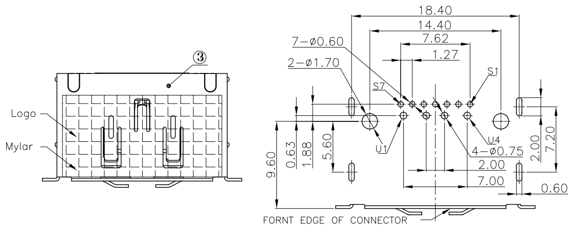
REFERENCE PC BOARD LAYOUT TOP VIEW (TOL=±0.05)
