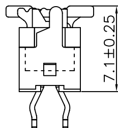
Mating Height Draw.
