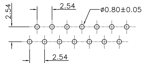
PCB Layout
