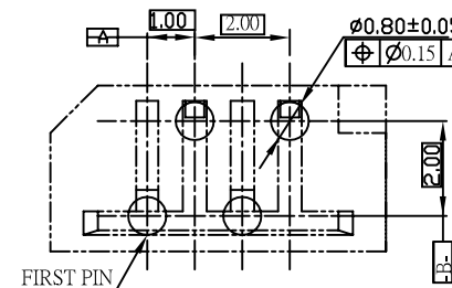
P.C.B. LAYOUT t=1.6\text{mm} COMPONENT SIDE
