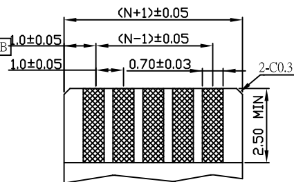
FPC THICKNESS=0.30mm TOLERANCE:0.05mm
