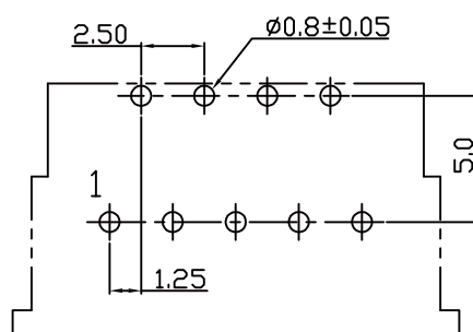
RECOMMEND PCB LAYOUT COMPONENT SIDE
