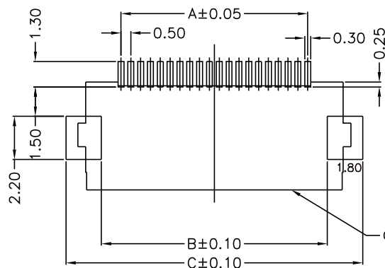
RECOMMENDED PCB LAYOUT COMPONENT SIDE
