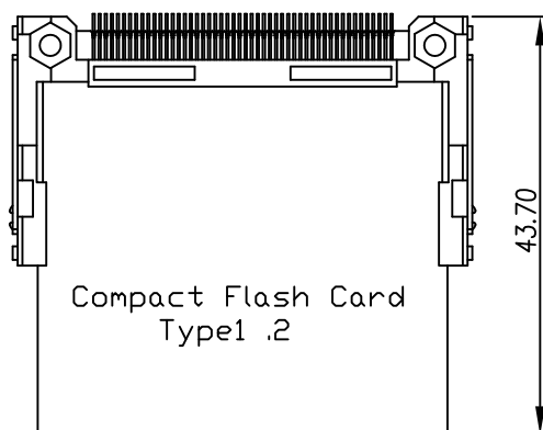
CARD INSERTION
