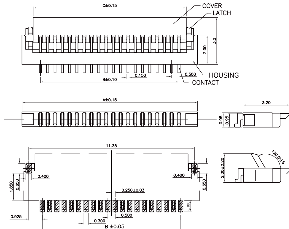
PCB Layout
