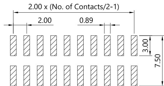
Recommended PCB Layout (PCB Board Tolerance ±0.05)
