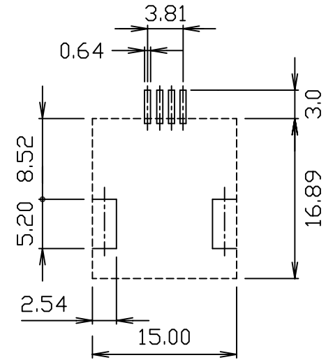
PCB LAYOUT
