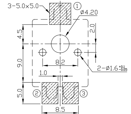
PCB LAYOUT(±0.1) (SOLDER PAD)
