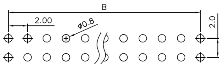
P.C. Board Layout (Tolerance: \pm 0.05 )
